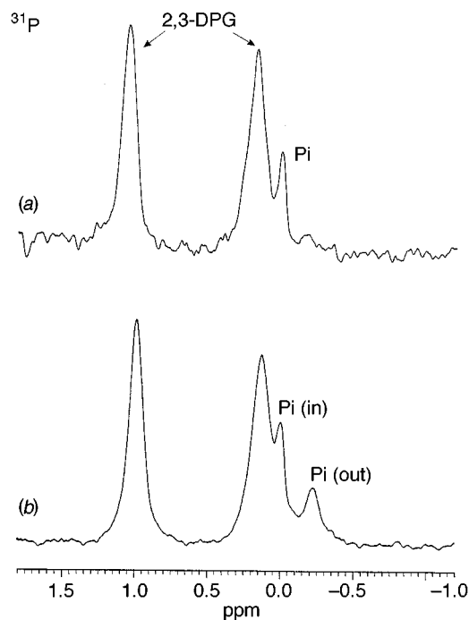
Fig. 19 ^{31}\text{P} NMR spectra of human blood before (a) and after (b) the addition of 5 mM of \text{Eu}(\text{DTMA})^{3+} (39 °C at 2.1 T) (2,3-DPG = 2,3-diphosphoglycerate; Pi = inorganic phosphate)
