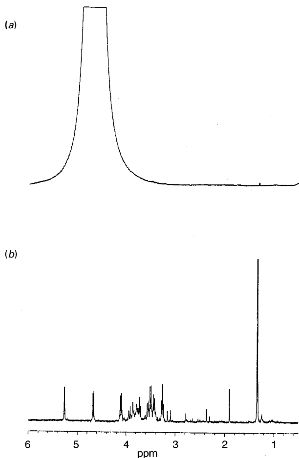
Fig. 20 ^1\text{H} -NMR spectra of normal human CSF in 95% \text{H}_2\text{O} -5% \text{D}_2\text{O} solution containing a 2.5 mM concentration of \text{Dy}^{\text{III}} -complex (25 ^\circ\text{C} at 9.4 T ). (a) single pulse method. (b) Carr-Purcell-Meiboom-Gill spin-echo spectrum.
